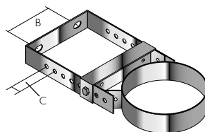
Wall Band and Adjustable Back Bracket Assembly
