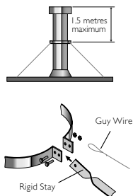
Telescopic Roof Stays
