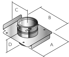
Fig.1 Top Plate
