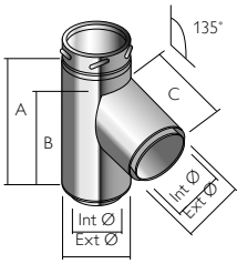
135° Tee
