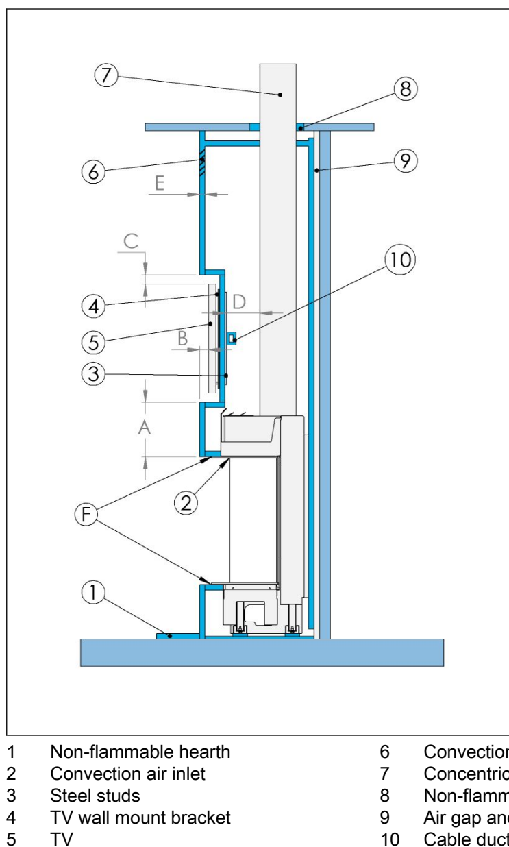
Figure 21. TV installation - flush mounted
