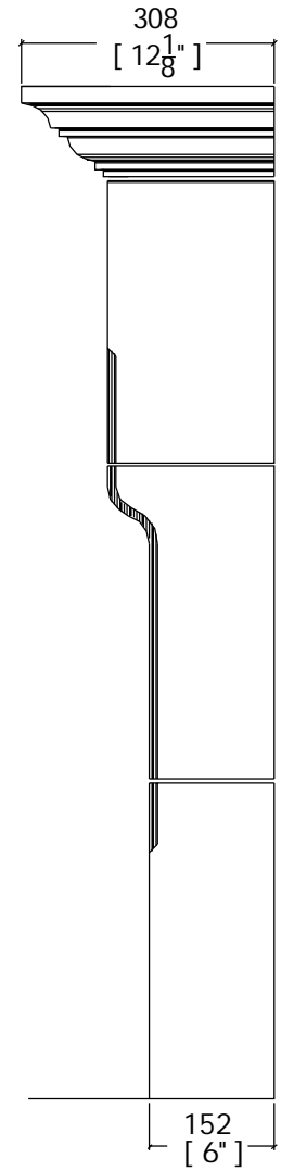
SIDE ELEVATION
