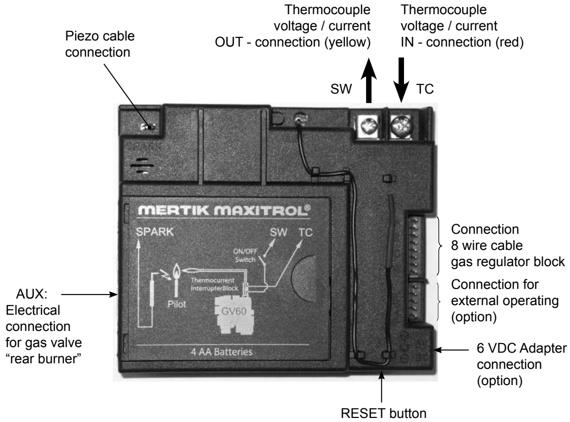
Figure 26: Receiver - Top
