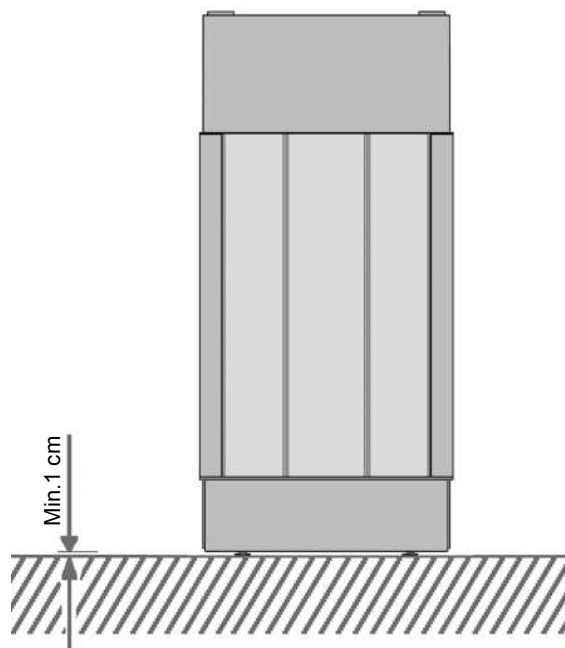
Figure 15: A clearance of at least 1 cm must be maintained between the bottom of the appliance and the floor.
