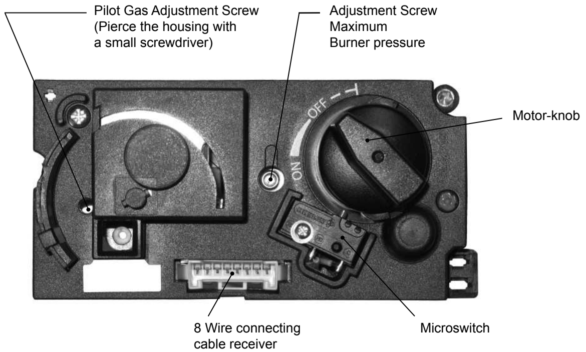
Figure 24: Gas regulator block - Front
