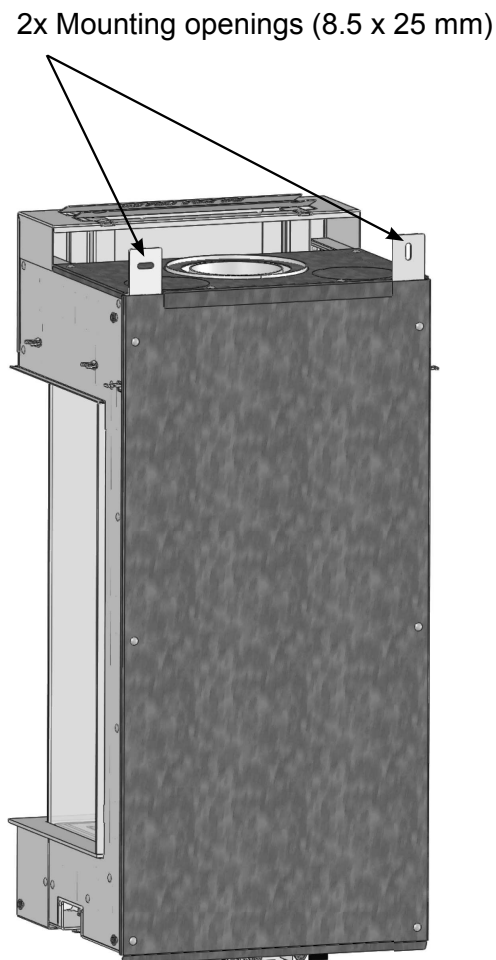
Figure 21: Mounting openings (2x) Rear Wall-mounted appliance
