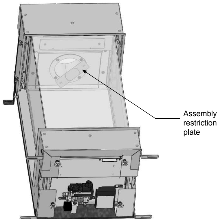
Figure 32: Positioning restriction plate
