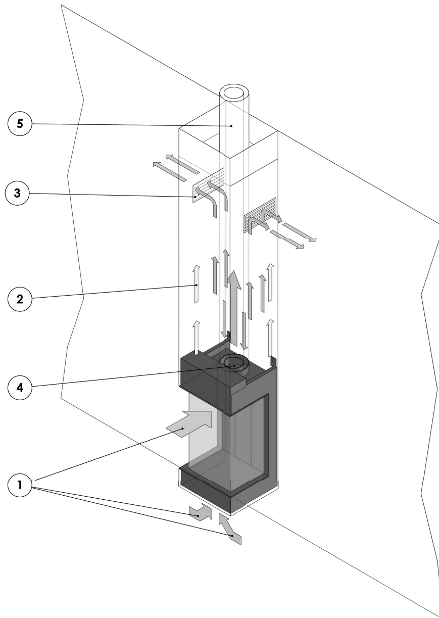
Figure 19: WALL-MOUNTED APPLIANCE: Appliance with ventilated cove Vertical outlet of the flue gas exhaust / combustion air supply via the roof. Fitted without convection package
