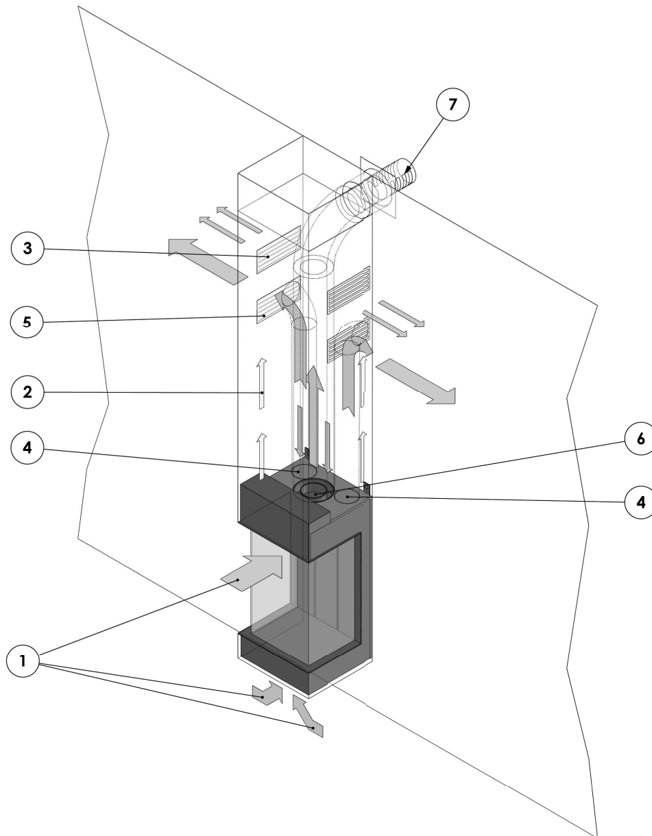
Figure 18: WALL-MOUNTED APPLIANCE: Appliance with ventilated cove Horizontal outlet of the flue gas exhaust / combustion air supply via the wall.
