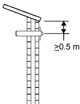
Figure 2: Wall-mounted outlet
